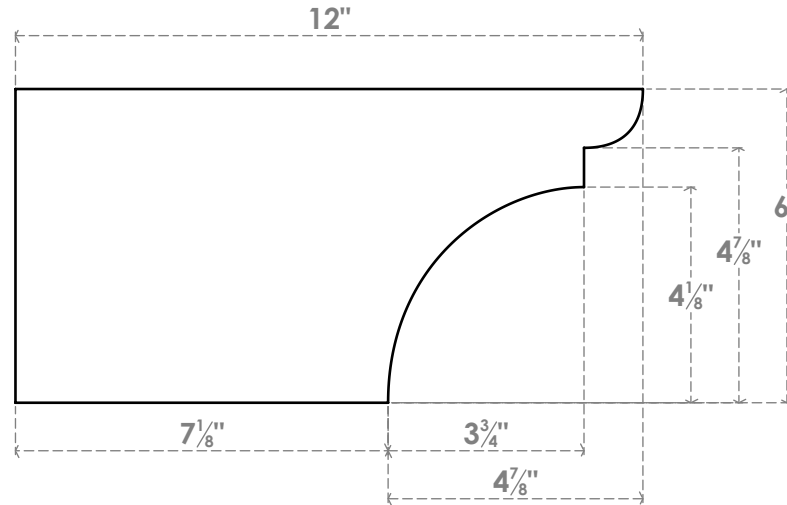
SIDE PROFILE
